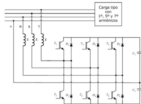
Fig. 1. Three-phase active filter topology
