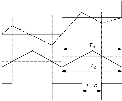
Fig. 3. Symmetric PWM technique
