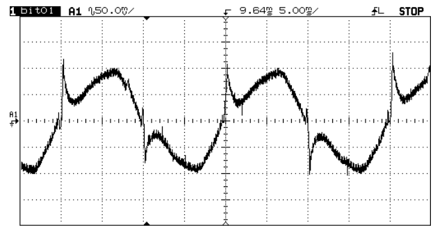
Fig. 14. Corrected source current with Adjustable PWM
