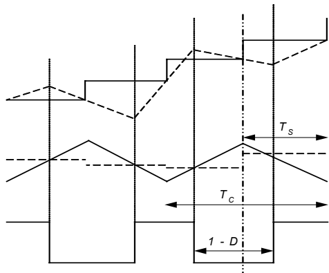
Fig. 4. Asymmetric PWM technique
