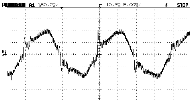
Fig. 13. Corrected source current with Asymmetric PWM
