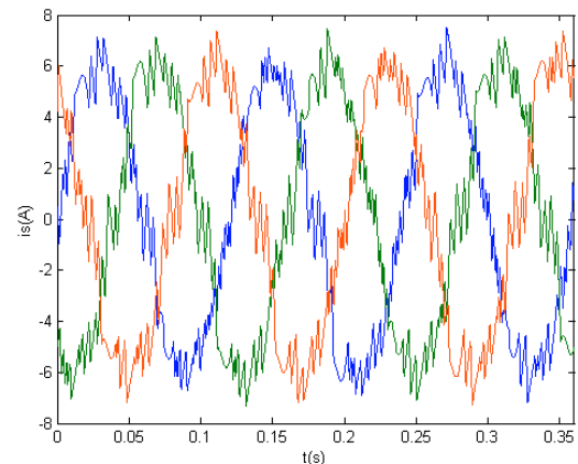
Fig. 7. Corrected Source Current with Adjustable PWM.
