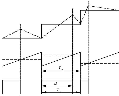
Fig. 2. Standard PWM technique
