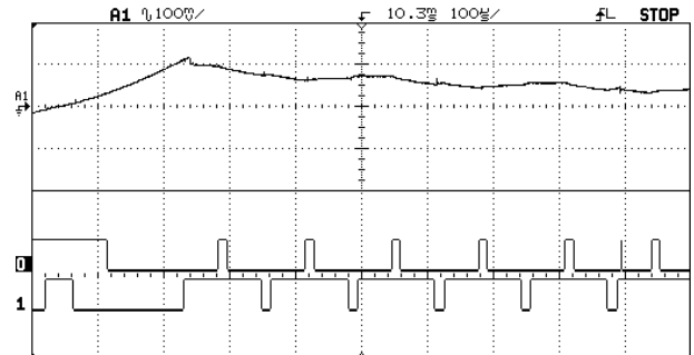
Fig. 15. Corrected source current and Control signals with Asymmetric PWM
