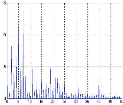
Fig.8. Standard PWM technique
