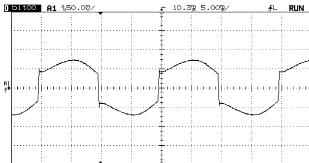
Fig. 12. Load current demanded by the rectifier
