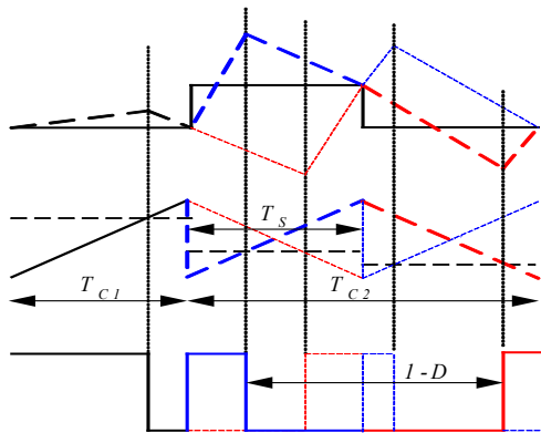
Fig. 5. Adjustable PWM technique
