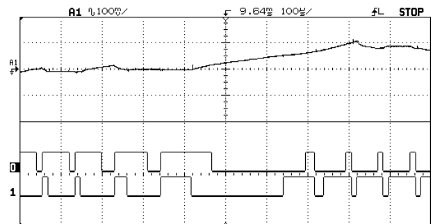
Fig. 16. Corrected source current and Control signals with Adjustable PWM
