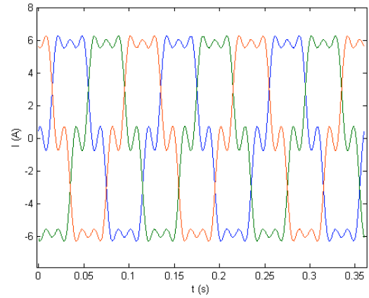
Fig. 6. Pattern Load Current
